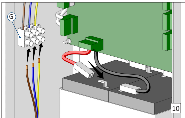
Connect the power supply cable to terminal "G". Connect the red cable to the battery.
