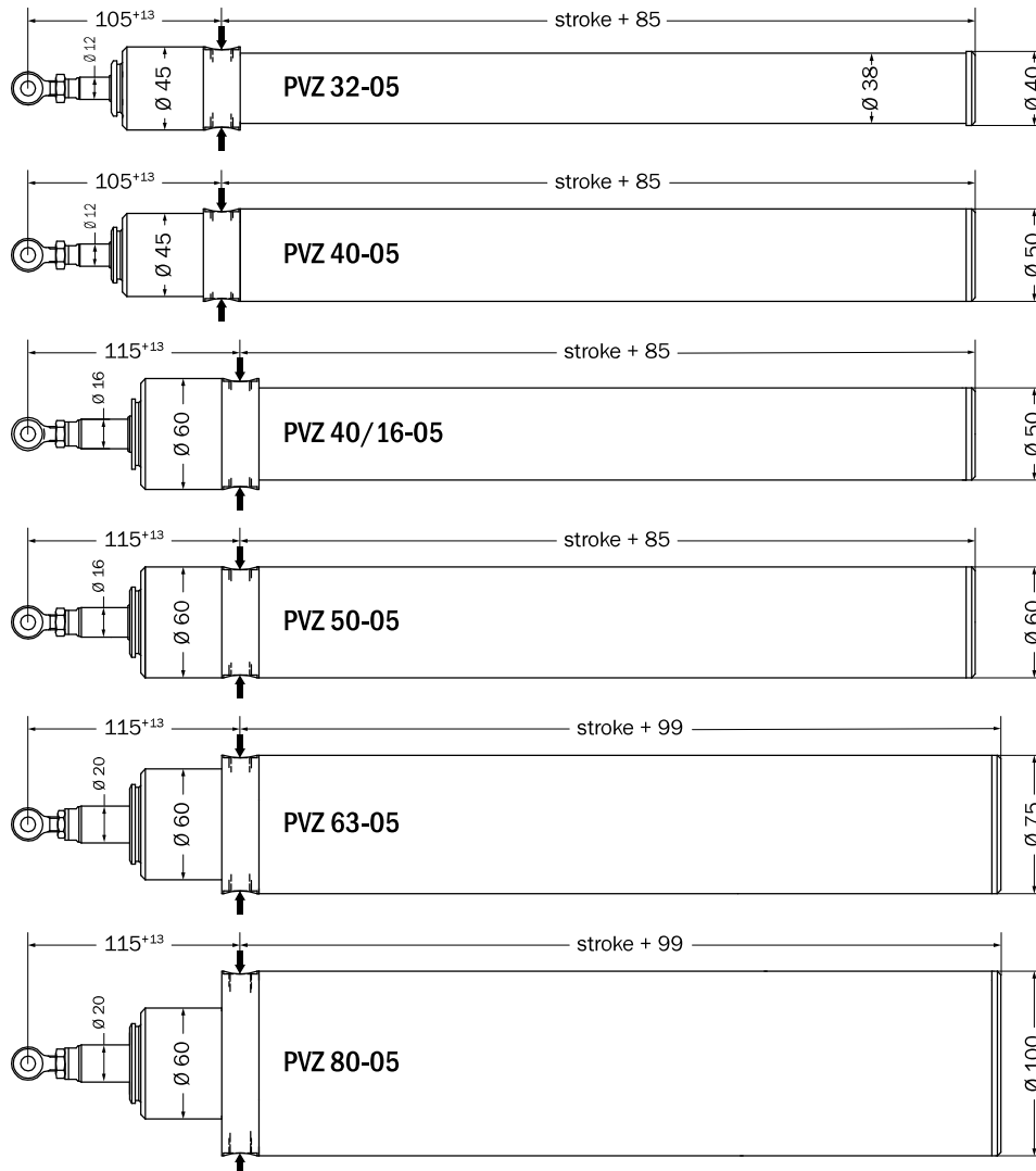
Illustration cylinder type 05
