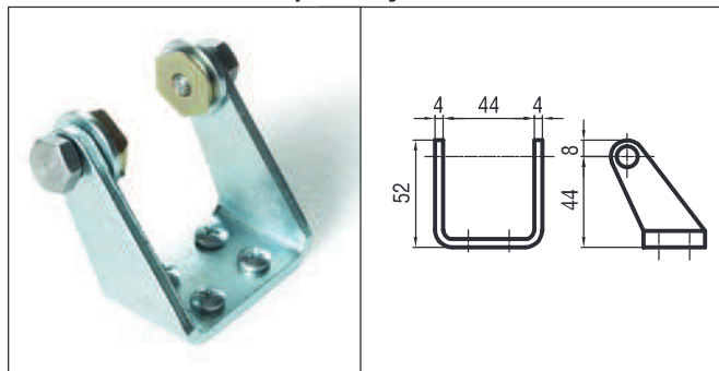
Galvanized steel sliding bracket part No. 40235F. It allows the fixing for the whole length of the actuator. To use only for single Rack.
