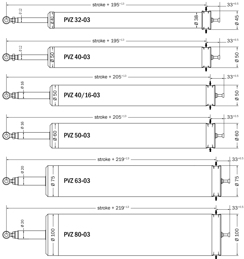
Illustration cylinder type 03
