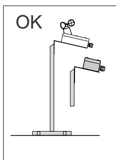
Post mounting
