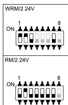
DIP-Switch indstilling
