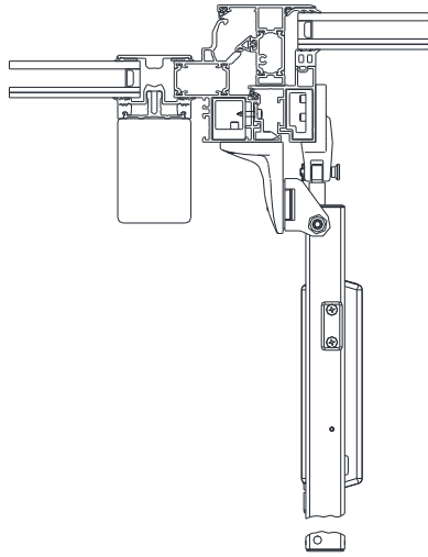
Raico® WING 105-DI
