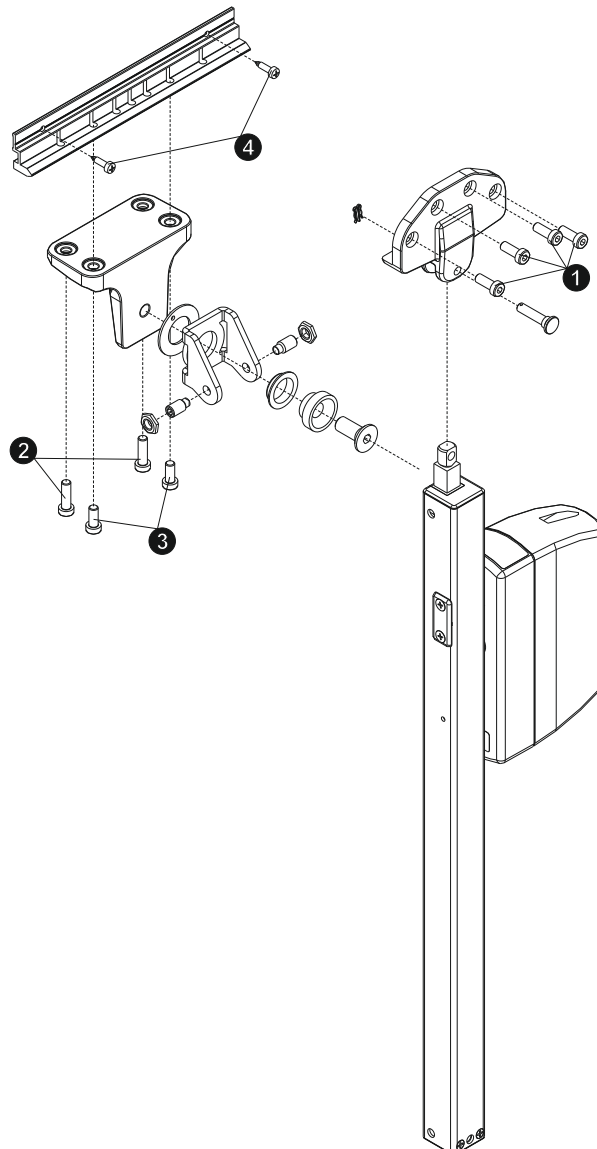
Raico® WING 105-DI
